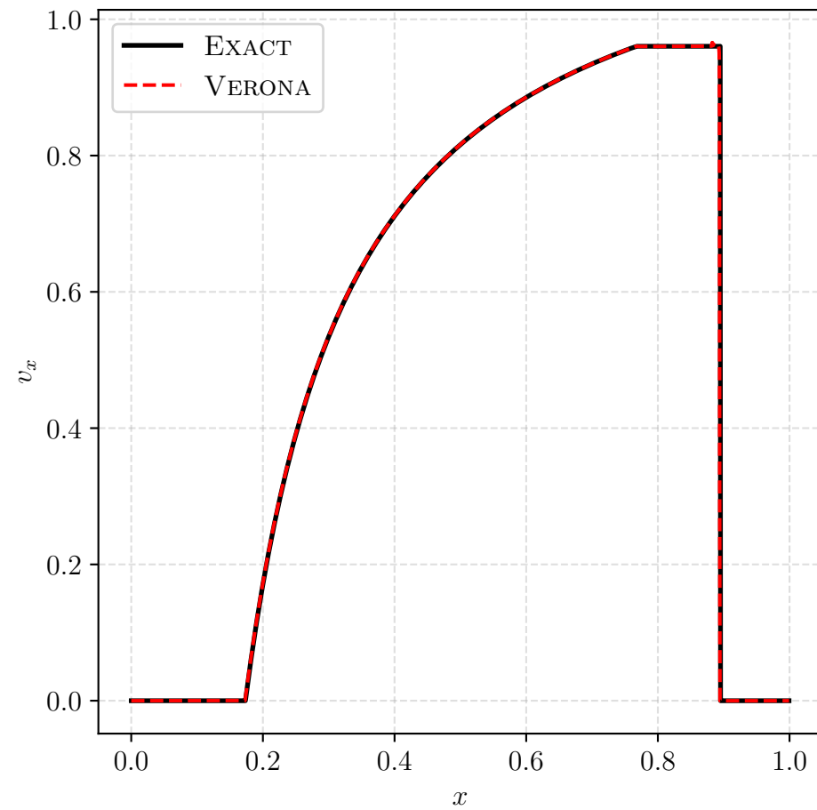
Shock Tube I
